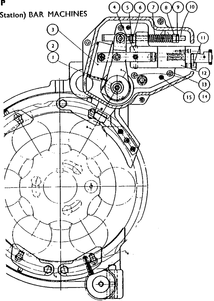
(Drawing No. 153 Z 1B)
