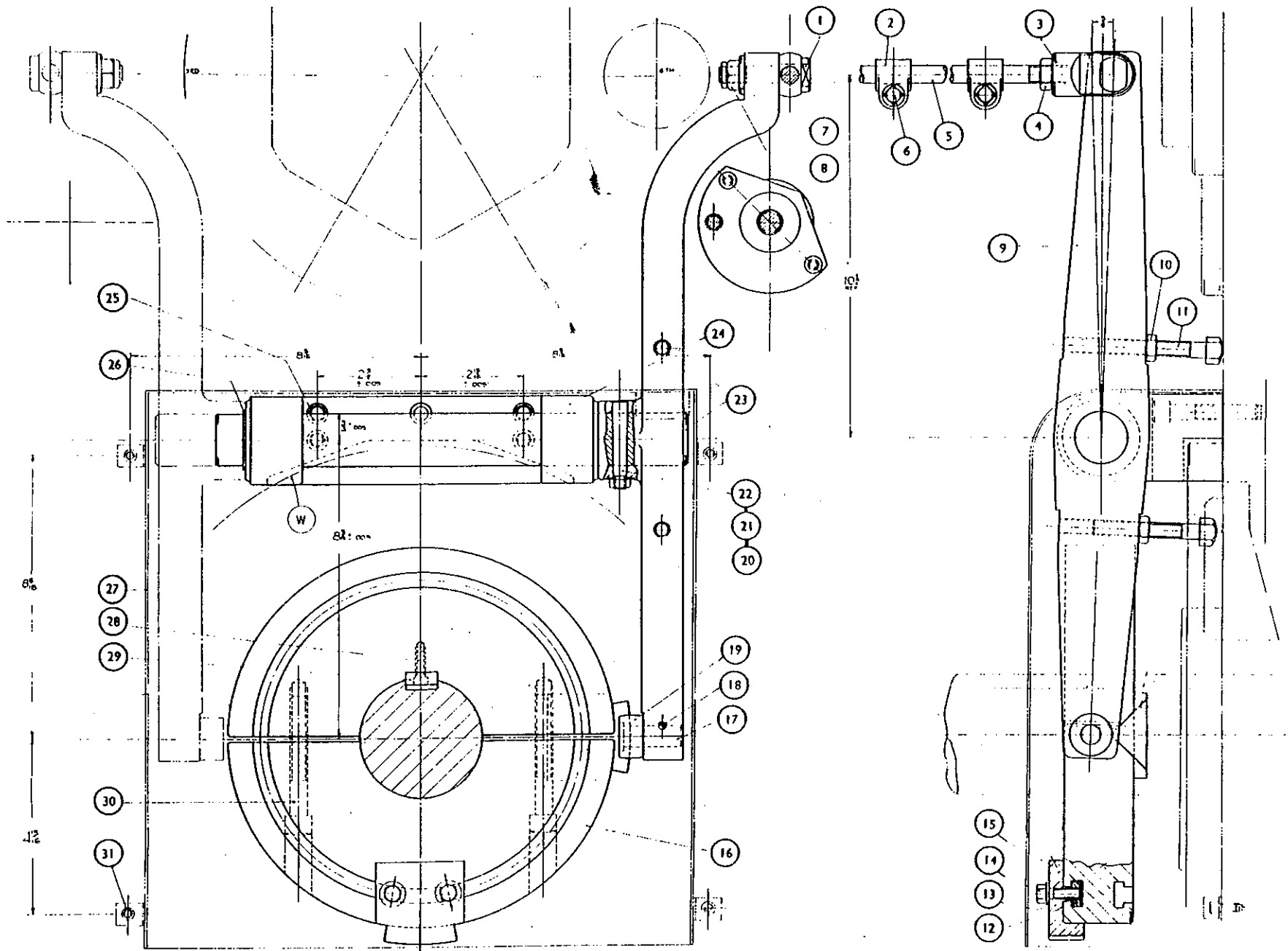
PLATE No.31 (Drawing No.A7584)
